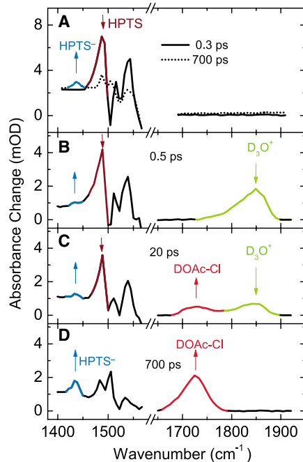
Fig. 1. Transient spectra showing the response of HPTS photoacid (brown, 1486\text{ cm}^{-1} ) and HPTS ^- photobase (blue, 1435\text{ cm}^{-1} ) marker modes in the electronically excited state in the fingerprint region and the DOAc-Cl (red, 1725\text{ cm}^{-1} ) and \text{D}_3\text{O}^+ (green, 1850\text{ cm}^{-1} ) bands for the case of HPTS only (no base) (A) and for HPTS with 1\text{ M } ^-\text{OAc-Cl} (B to D) in \text{D}_2\text{O} . OD, optical density.
